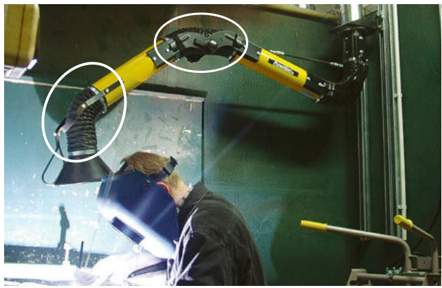
Exterior friction joints ("ClearThru" design), which allows for maximum air velocity, low pressure drop and low noise level
